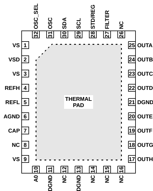
EL5126 (32 LD 5X6 QFN) TOP VIEW
