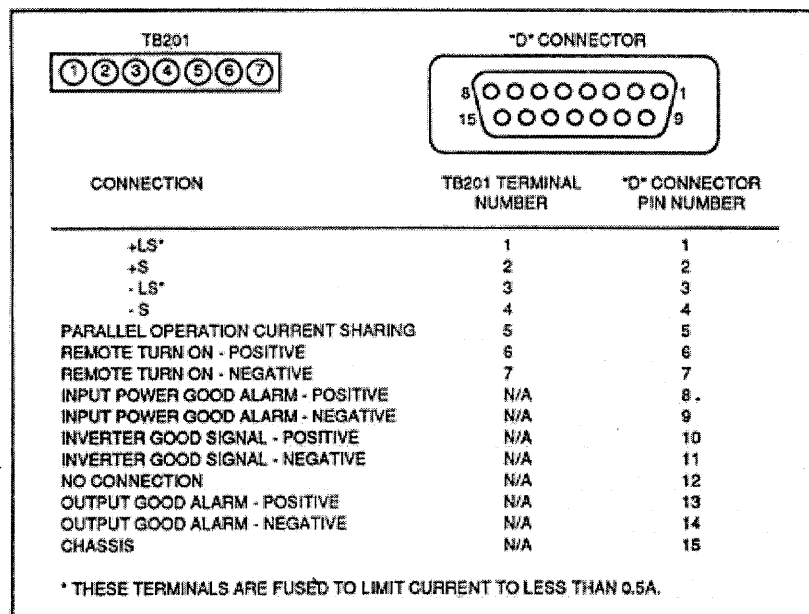
FIGURE 1: PINOUT FOR TB201 AND CHASSIS MOUNTED "D" CONNECTOR
