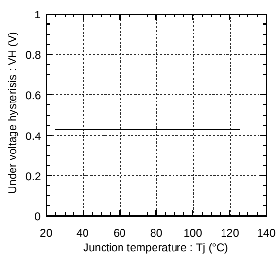
Under voltage hysteresis vs. Jnction temperature (typ.)
