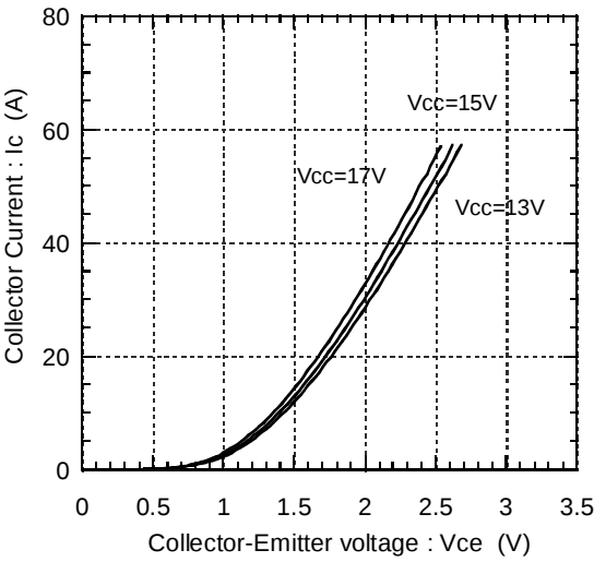
Collector current vs. Collector-Emitter voltage (typ.) Tj=25°C
