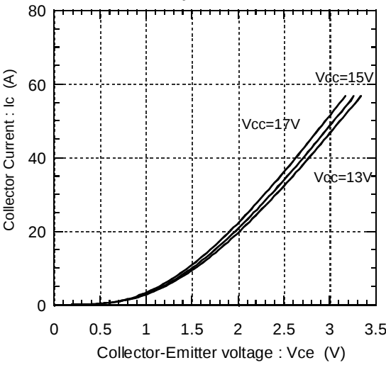
Collector current vs. Collector-Emitter voltage (typ.) Tj=125°C
