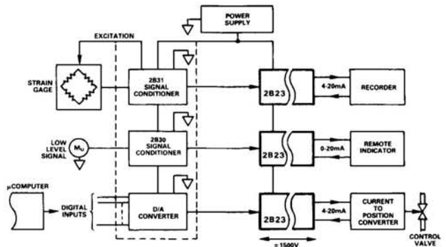
Figure 6. Multiloop Isolation
