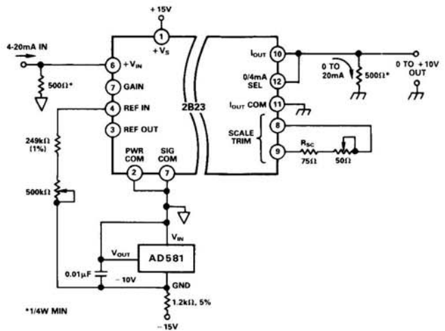
Figure 7. 4-20mA to 0 to +10V Isolated Converter
