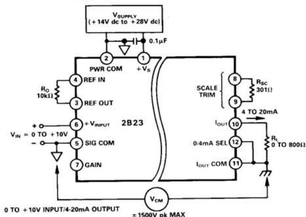
Figure 2. Basic Interconnections
