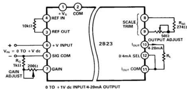
Figure 3. Input Gain Adjustment
