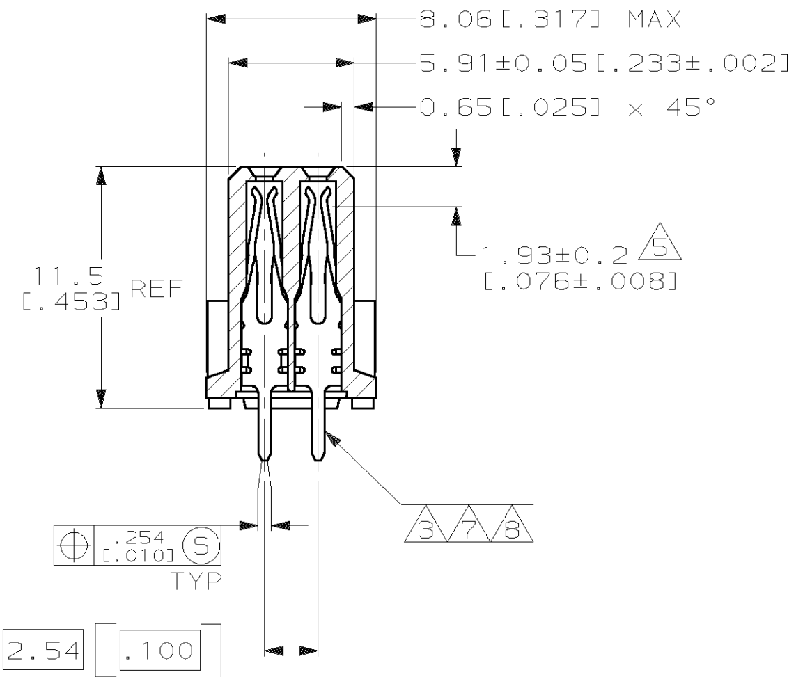
SECTION X-X
