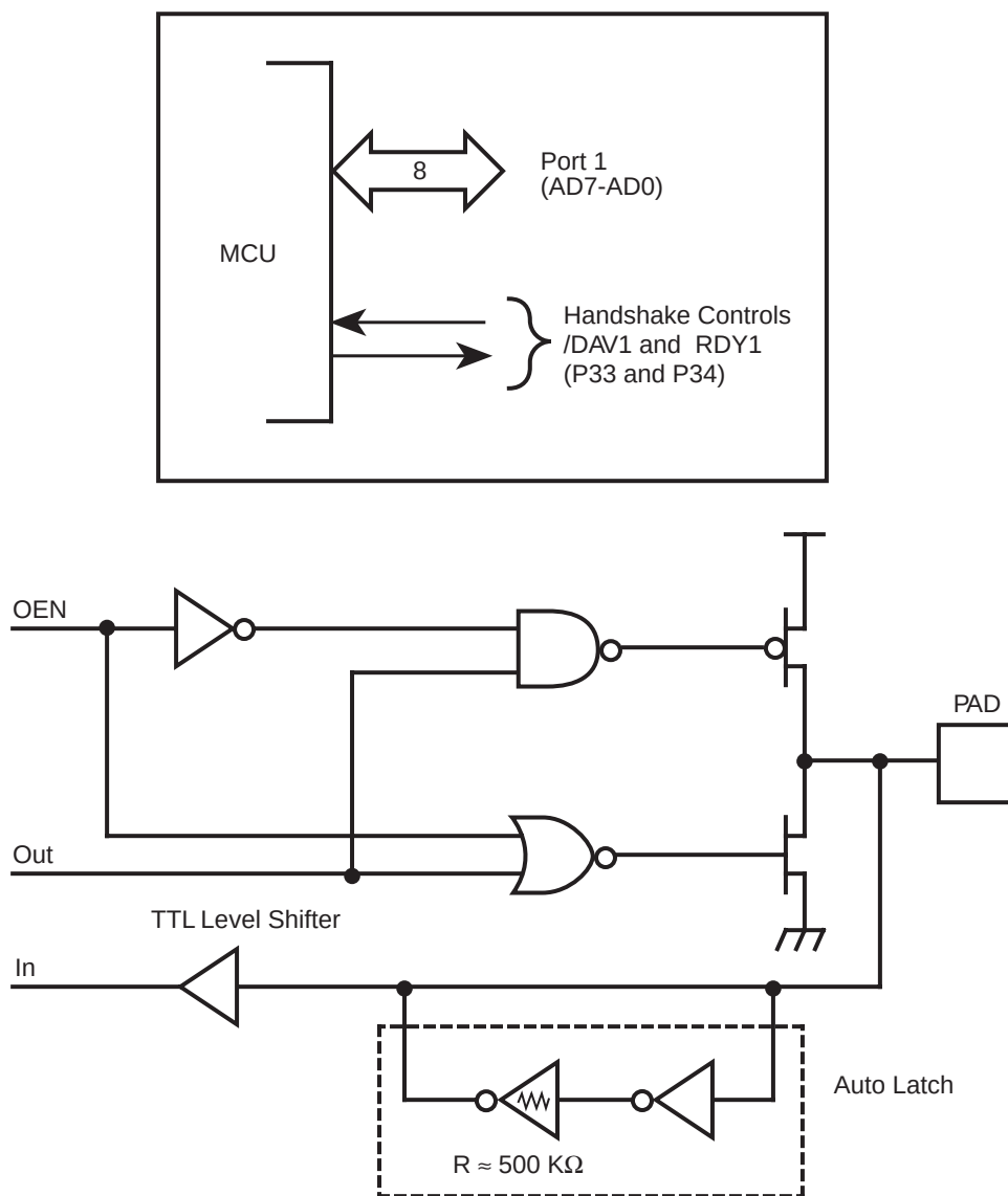
Figure 11. Port 1 Configuration
