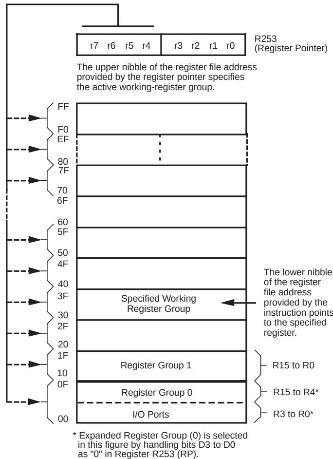
Figure 21. Register Pointer
