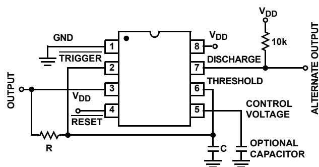
FIGURE 4. ASTABLE OPERATION
