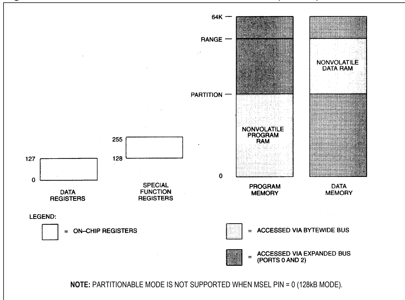
Figure 3. MEMORY MAP IN PARTITIONABLE MODE (PM = 0)
