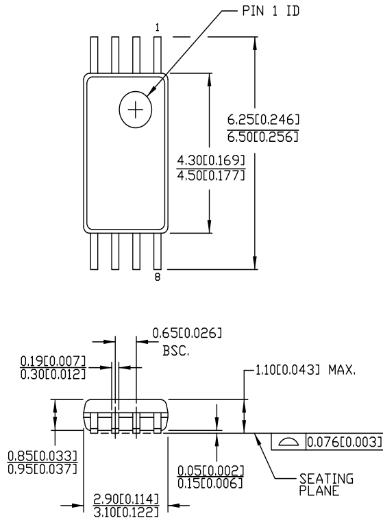
Figure 7. 8-pin TSSOP (4.40 mm Body) Z08.173/ZZ08.173 Package Outline, 51-85093
