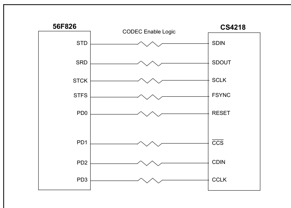
Figure 2-11. CS4218 Stereo Audio Codec
