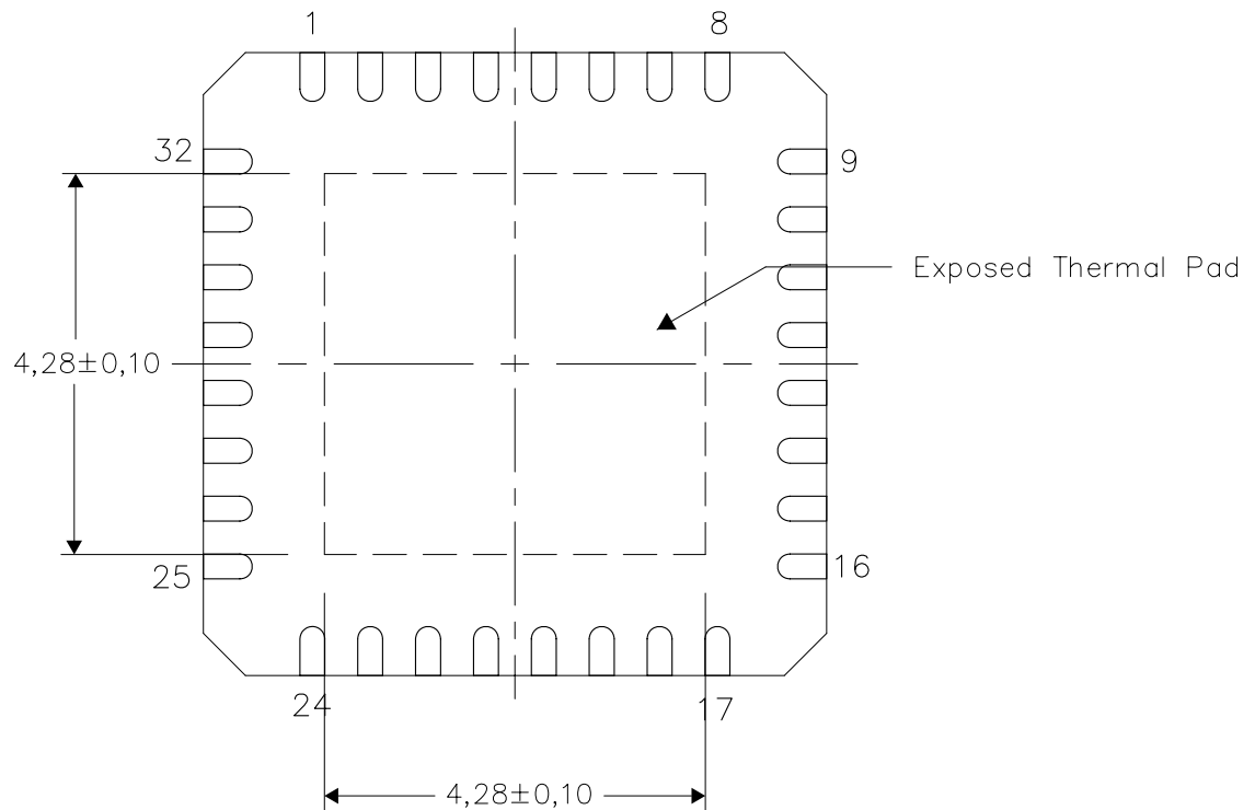
Bottom View
