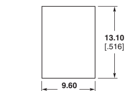
Recommended Panel Cutout Max. Panel Thk. 1.7 [0.067]
