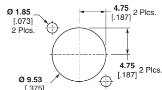
Recommended Panel Cutout Max. Panel Thk. 1.70 [0.067]
