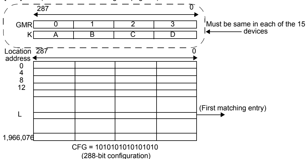
Figure 10-61. ×288 Table with Fifteen Devices
