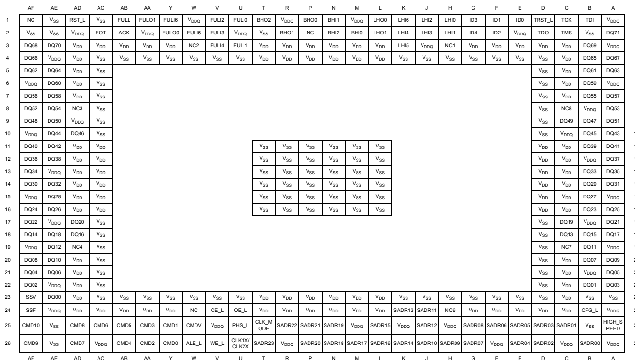
Figure 18-1. Pinout Diagram
