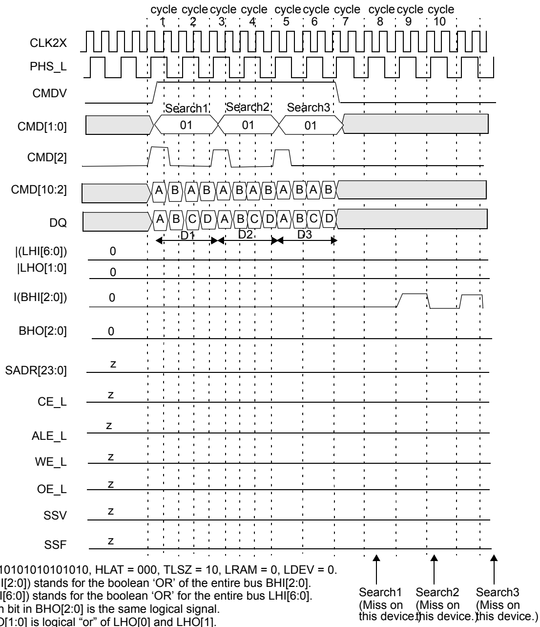
Figure 10-57. Timing Diagram for Devices Above the Winning Device in Block Number 3
