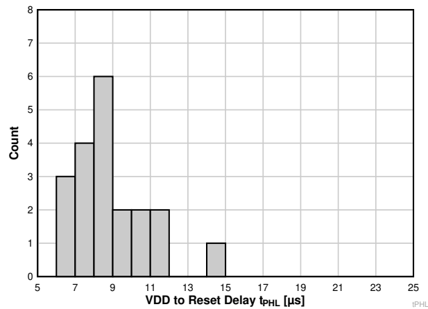
Figure 6-16. VDD to Reset Delay Histogram for TPS3823A-33 Devices at 25°C (Unit Count = 20)
