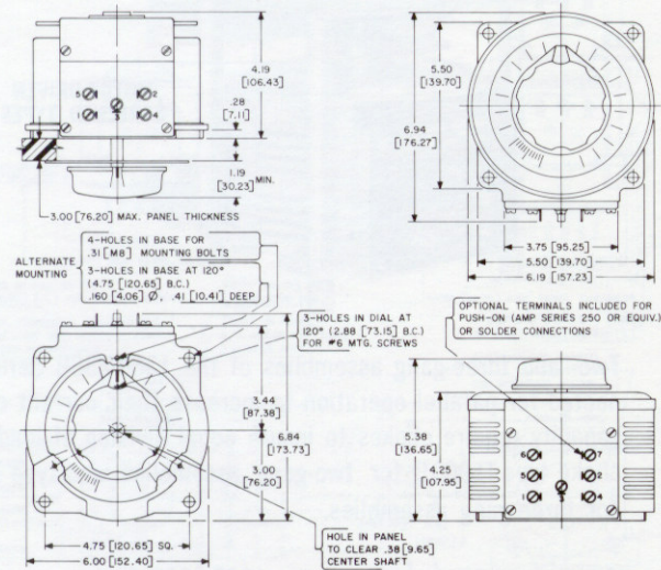
PANEL MOUNTED
