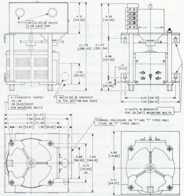
MOTOR DRIVEN
