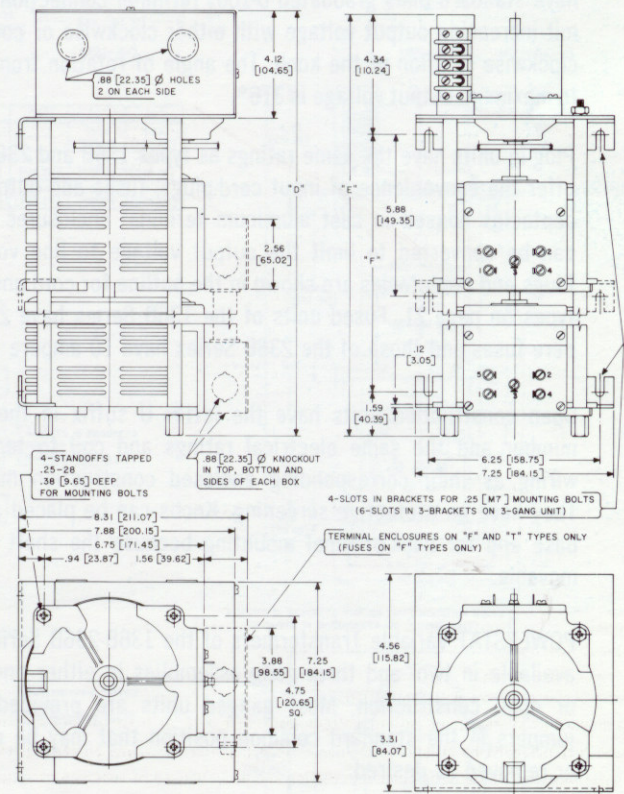
MOTOR DRIVEN
