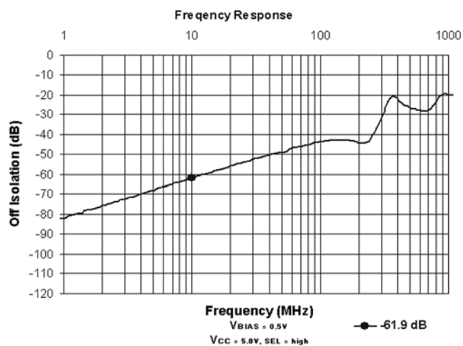
FIGURE 4. OFF Isolation
