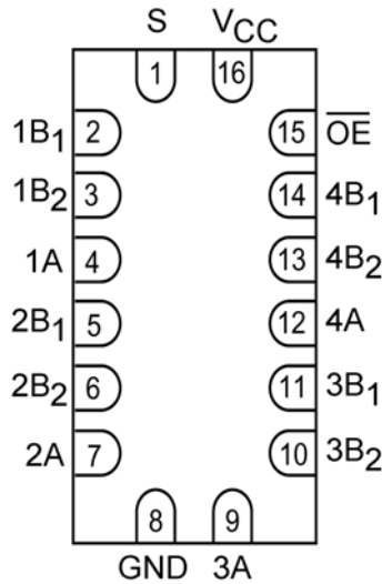
Pad Assignments for DQFN (Preliminary)
