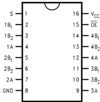
Pin Assignments for QSOP and TSSOP
