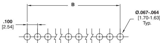
Recommended PC Board Hole Layout
