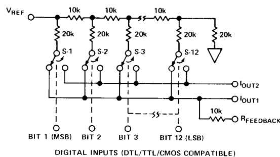
Figure 5. AD7541 Functional Diagram (Inputs "HIGH")
