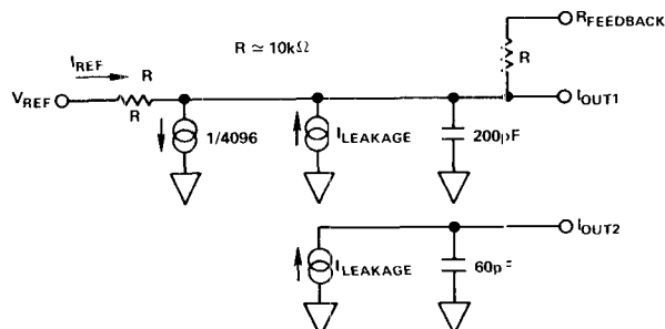
Figure 8. AD7541 Equivalent Circuit – All Digital Inputs High
