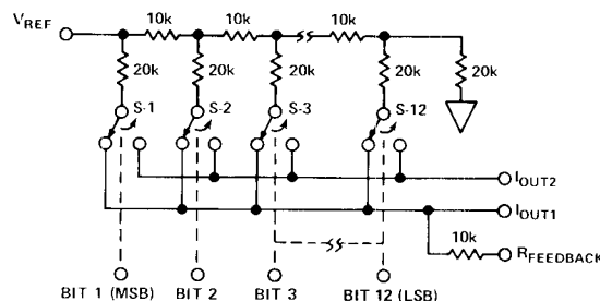
FUNCTIONAL DIAGRAM
