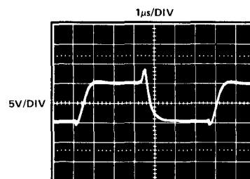
Figure 12. Output Waveform
