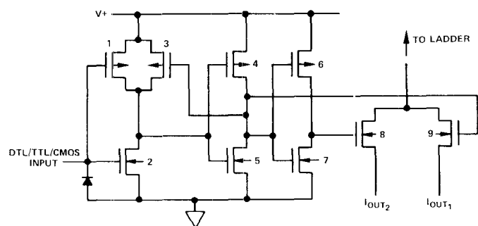
Figure 6. CMOS Switch
