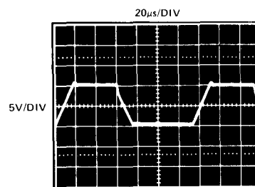
Figure 10. Output Waveform
