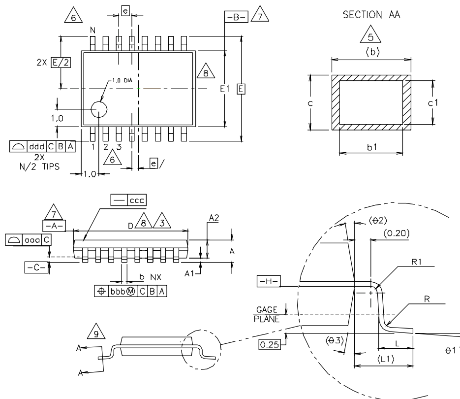
Figure 36. TSSOP-28 Package
