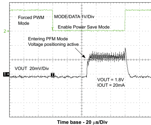
Figure 26. Forced PWM/PPM Mode Transition
