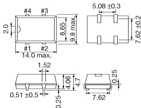
Figure 1) ECS-8FX Top and Side view
