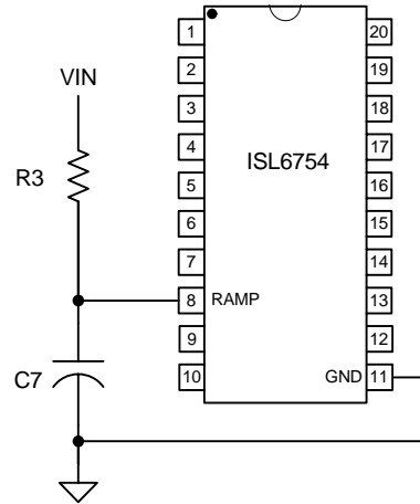
FIGURE 9. VOLTAGE FEED FORWARD CONTROL
