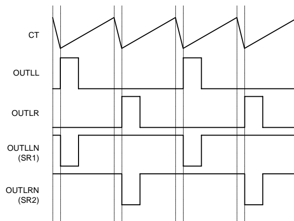
FIGURE 20. BASIC WAVEFORM TIMING
