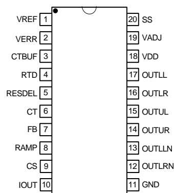
ISL6754 (20 LD QSOP) TOP VIEW
