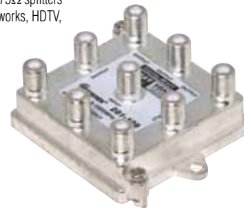
201-108 8-Way 1GHz 130dB RF Balanced Digital Splitter
