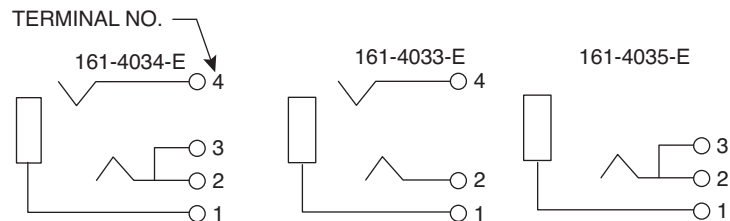
CIRCUIT DIAGRAMS
