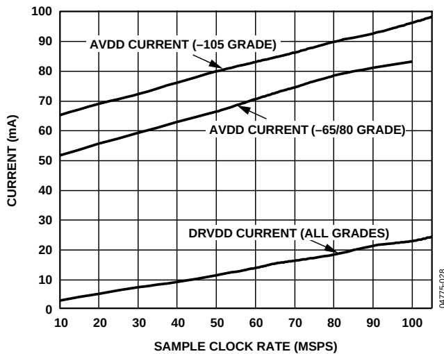
Figure 23. I_{AVDD} , I_{DRVDD} vs. Sample Clock Frequency, C_{LOAD} = 5 pF, A_{IN} = 70 MHz @ –0.5 dBFS
