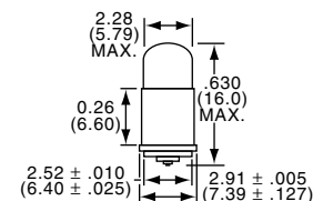
FLANGE BASE- T1 3/4
