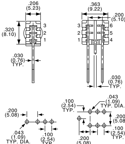
TT11DGVRA3T Vertical Actuation
