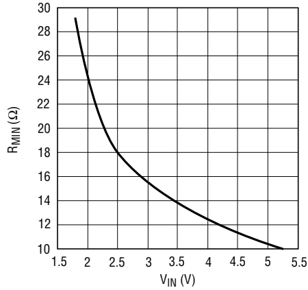
Start-Up into Resistive Load L = 10μH
