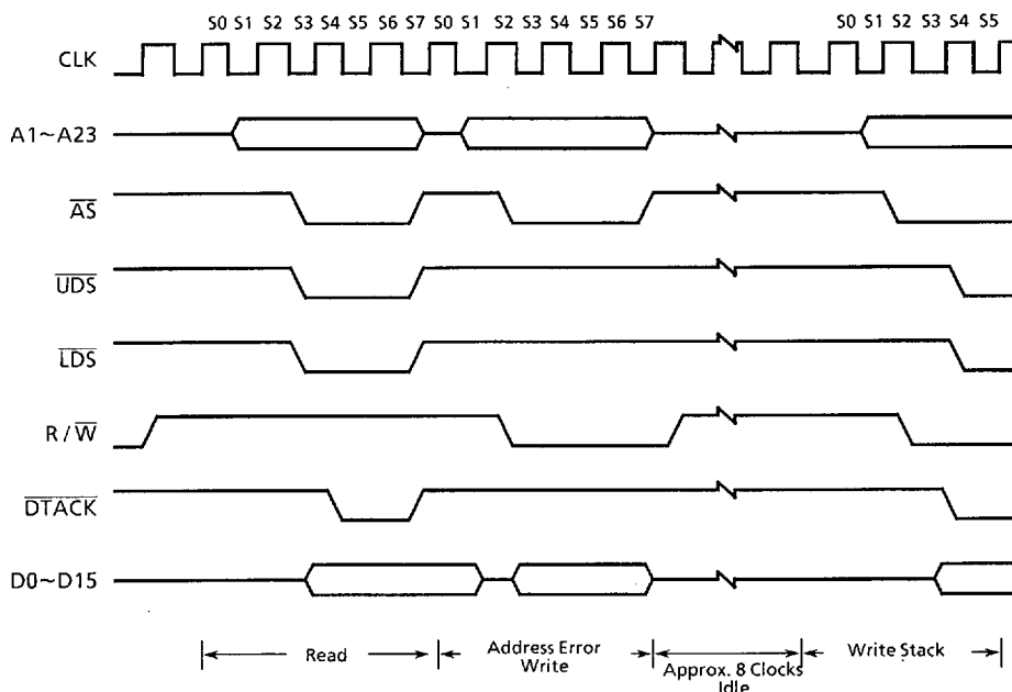
Figure 5.9 Address Error Timing Diagram
