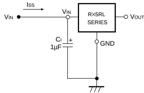
FIG. 3 Quiescent Current Test Circuit
