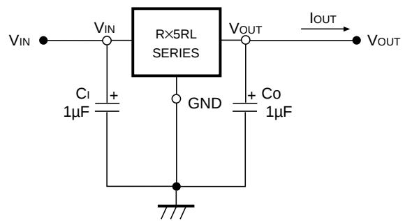
FIG. 2 Test Circuit
