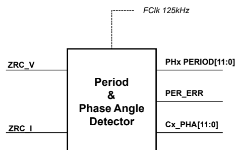
Figure 41. Phase meter
