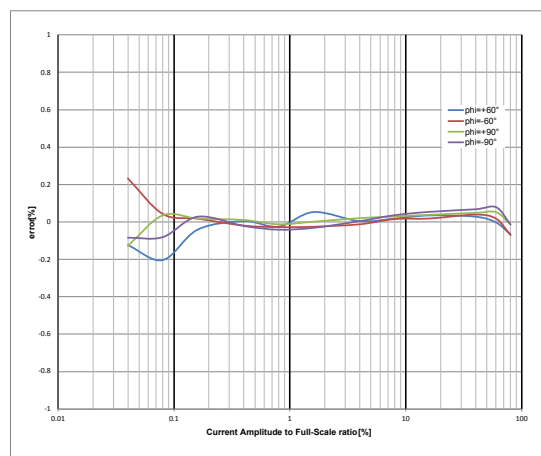
Figure 17. Reactive energy error vs. current gain=16x integrator off
