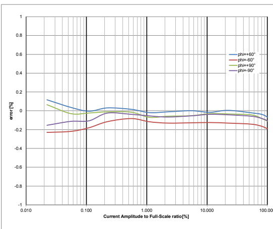
Figure 21. Reactive energy error vs. current gain=16x integrator on
