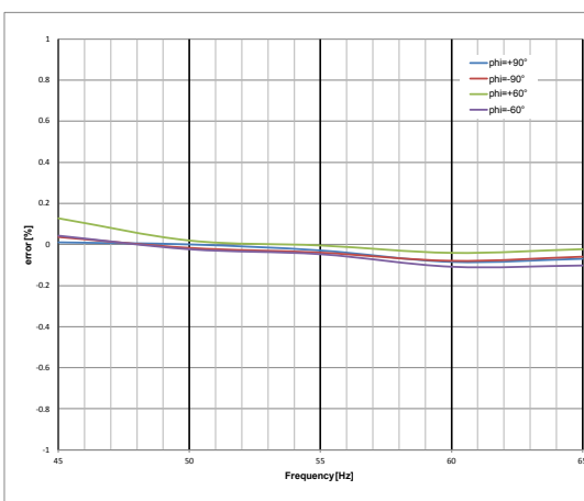
Figure 19. Reactive energy error vs. frequency gain=16x integrator off
