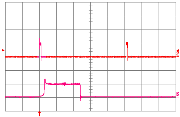
Fig. 2.5V.18: Load current (top trace, 20 A/div., 20 ms/div.) into a 10 \text{ m}\Omega short circuit during restart, at V_{in} = 24\text{V} . Bottom trace (20 A/div., 1 ms/div.) is an expansion of the on-time portion of the top trace.
