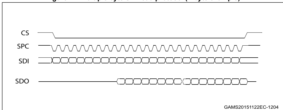
Figure 17. Multiple byte SPI read protocol (2-byte example)
