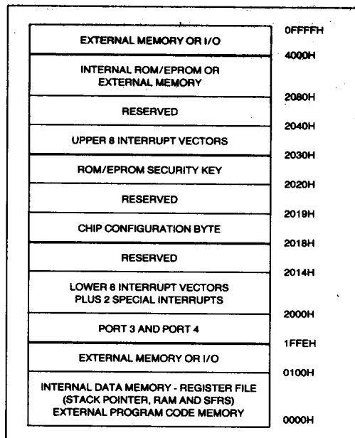
Figure 2. Memory Map
