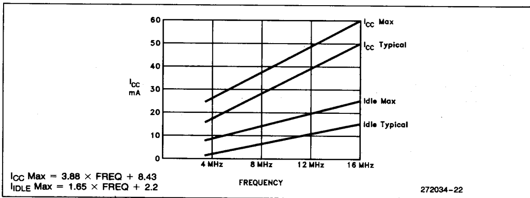
Figure 6. I_{CC} and I_{IDLE} vs Frequency
