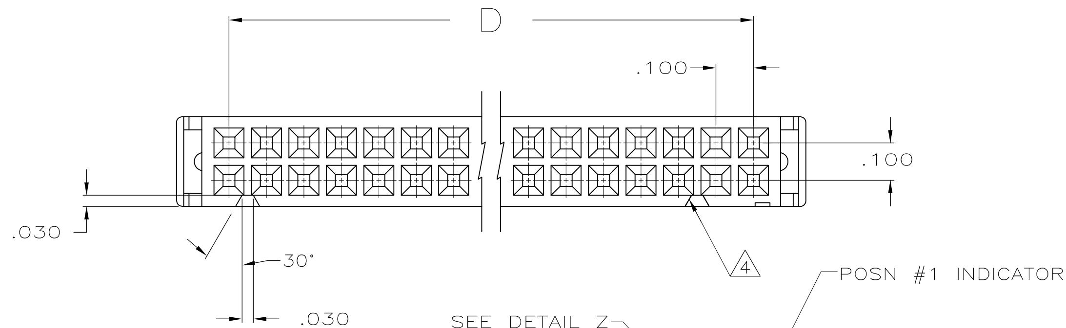
TERMINATED VIEW
