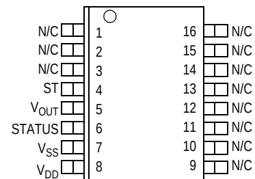
Figure 2. Pin Connections
