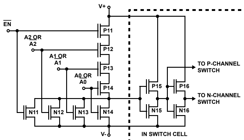
ADDRESS DECODER
