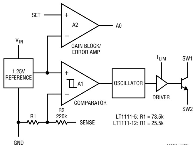
LT1111-5/LT1111-12
