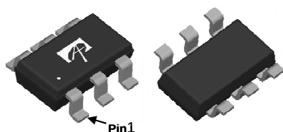
TSOP6 Top View Bottom View
