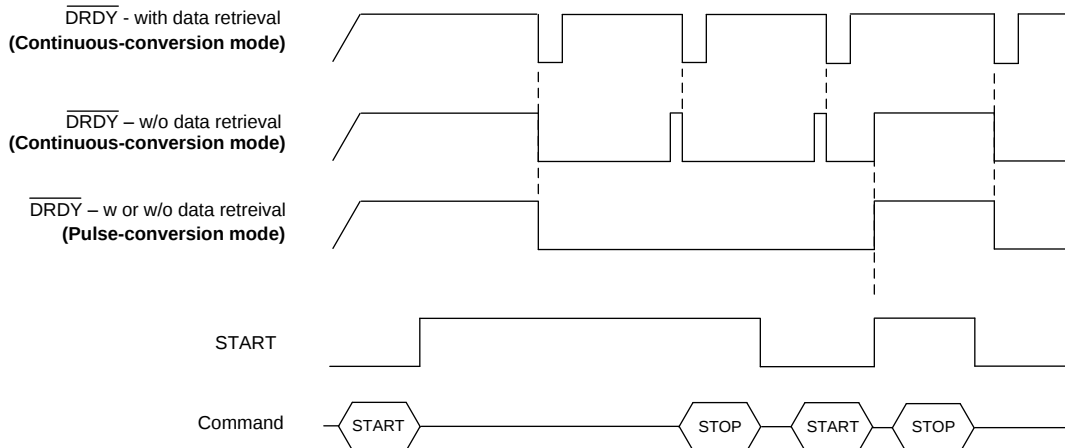
Figure 61. \overline{\text{DRDY}} Operation
