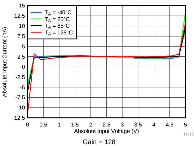
Figure 29. Absolute Input Current
