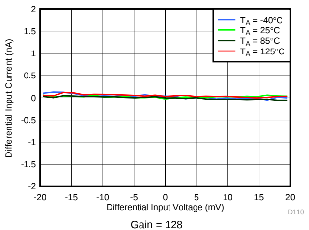
Figure 26. Differential Input Current
