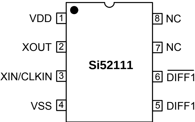
Figure 7. 8-Pin TSSOP
