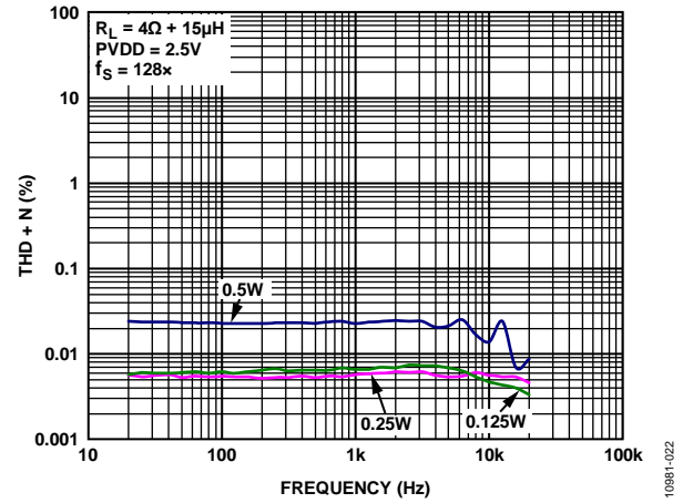
Figure 19. THD + N vs. Frequency, PVDD = 2.5\text{ V} , R_L = 4\ \Omega , f_s = 128\times
