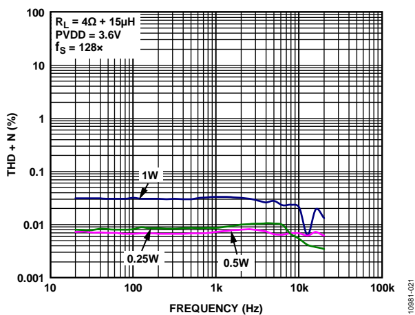
Figure 18. THD + N vs. Frequency, PVDD = 3.6\text{ V} , R_L = 4\ \Omega , f_s = 128\times
