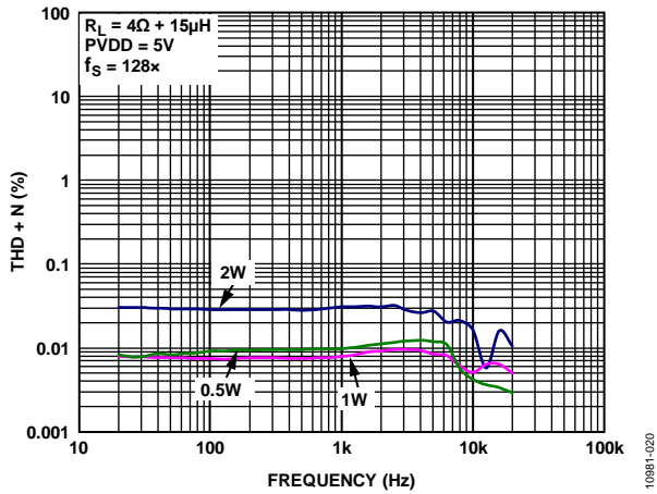
Figure 17. THD + N vs. Frequency, PVDD = 5\text{ V} , R_L = 4\ \Omega , f_s = 128\times
