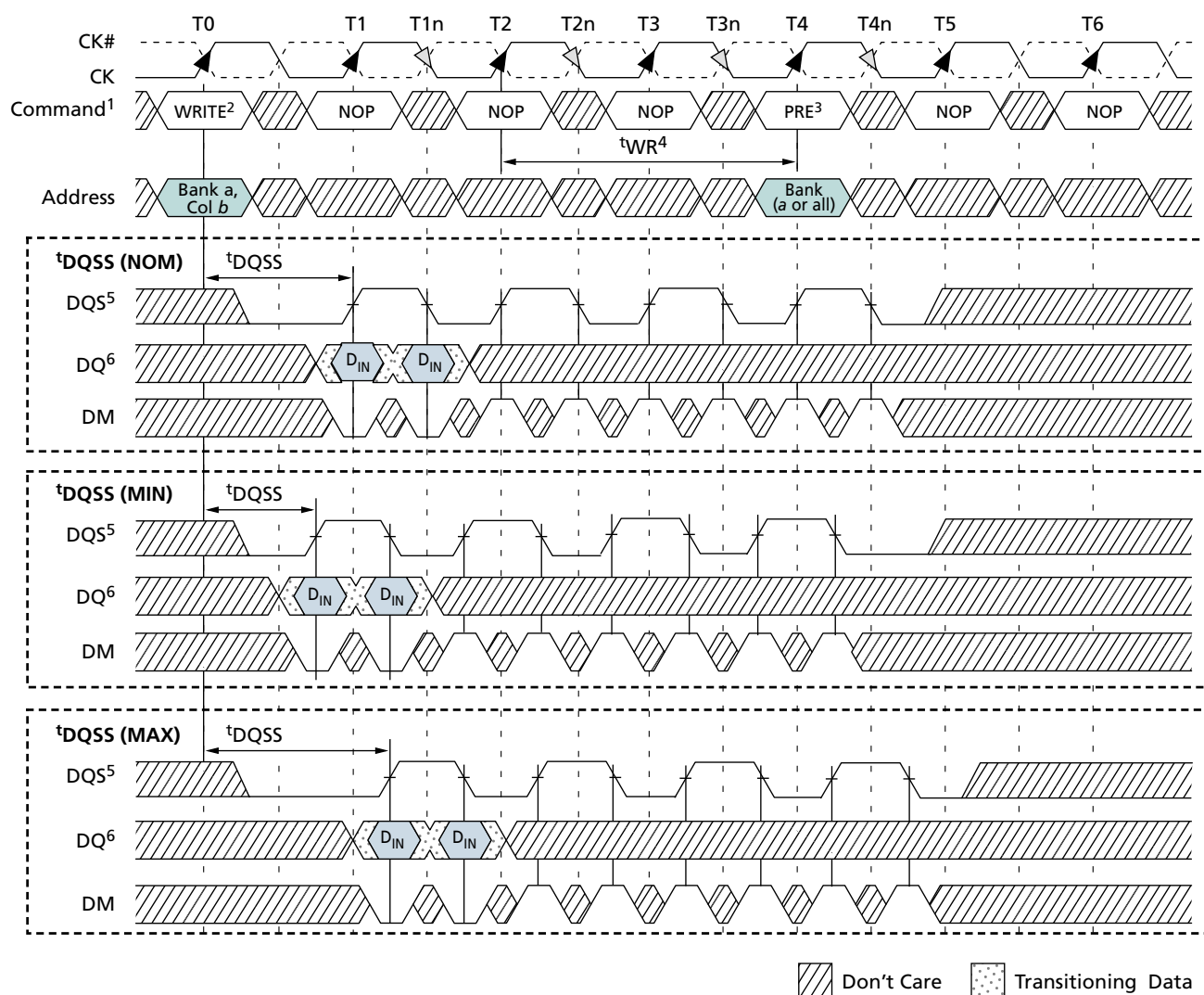
Figure 43: WRITE-to-PRECHARGE – Interrupting
