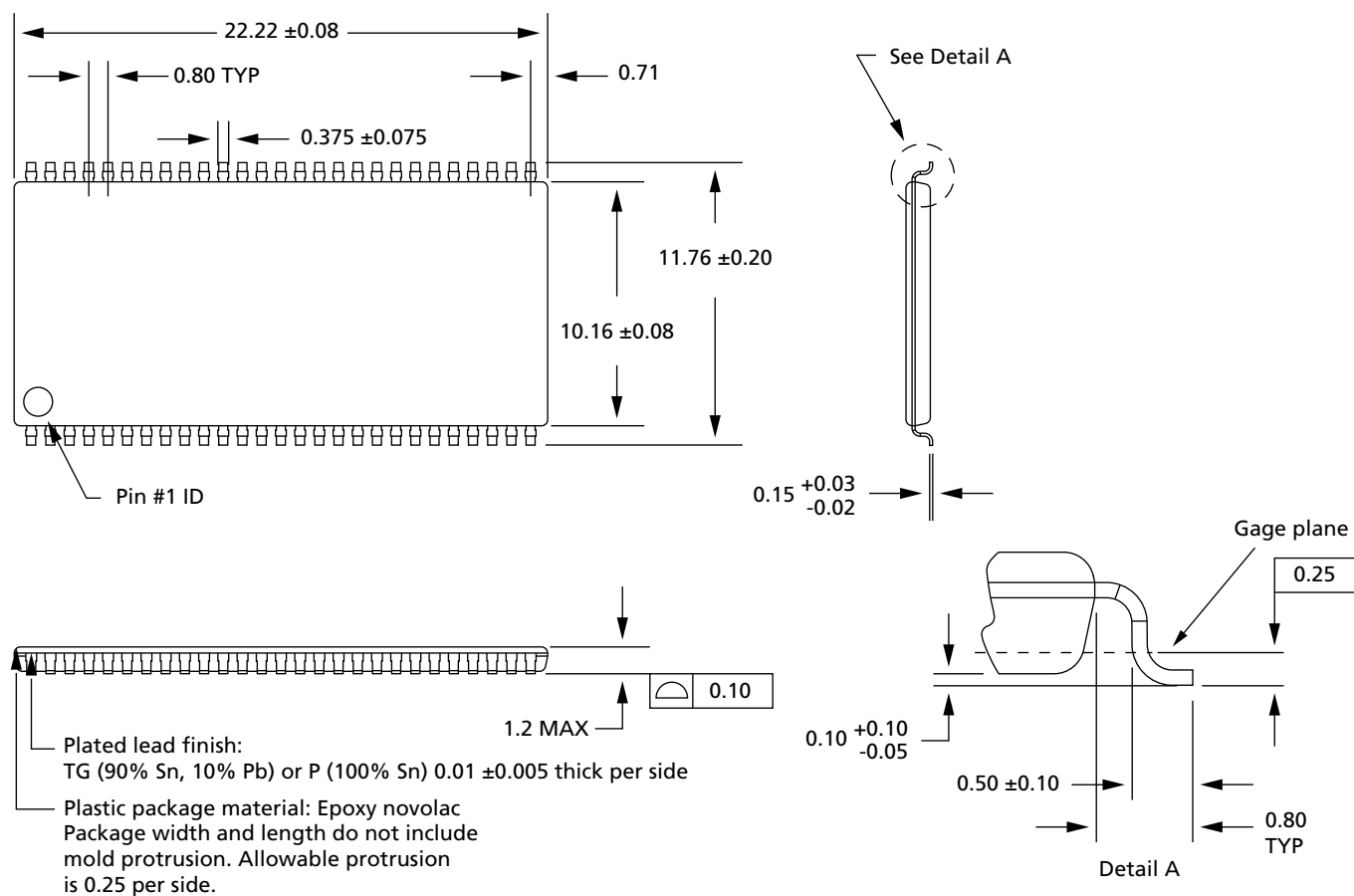
Figure 7: 54-Pin Plastic TSOP (400 mil) – Revision L
