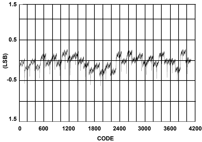
FIGURE 6. TYPICAL INL
