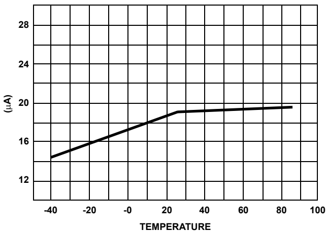
FIGURE 8. OFFSET CURRENT OVER TEMPERATURE
