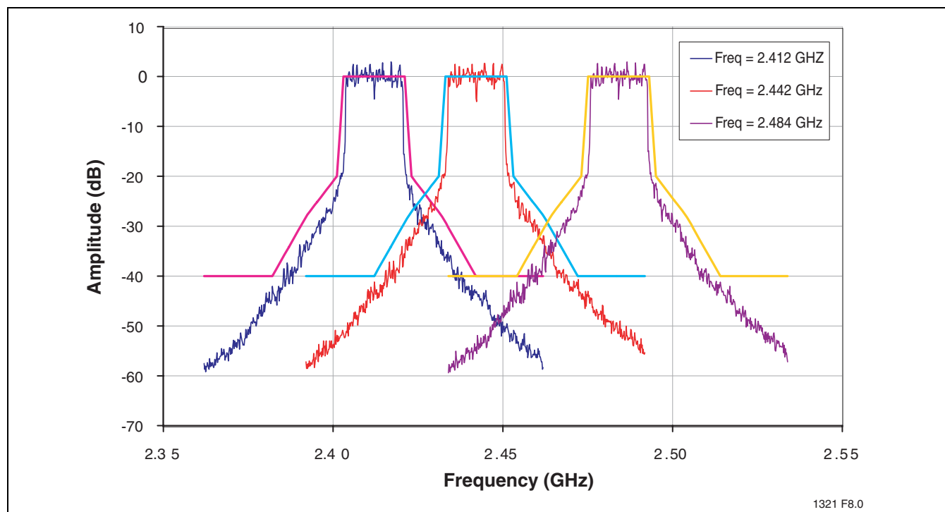
FIGURE 8: 802.11g Spectrum Mask at 22 dBm
