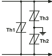
Figure 32. MULTI-POINT PROTECTION
