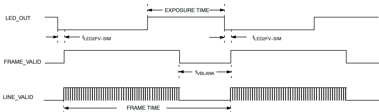
Figure 14. Simultaneous Master Mode Synchronization Waveforms #1
