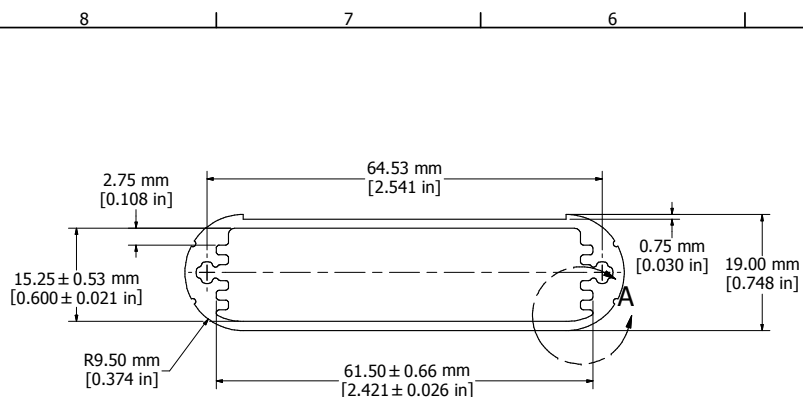
EXTRUSION
