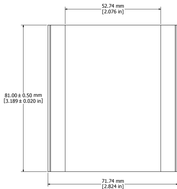
EXTRUSION
