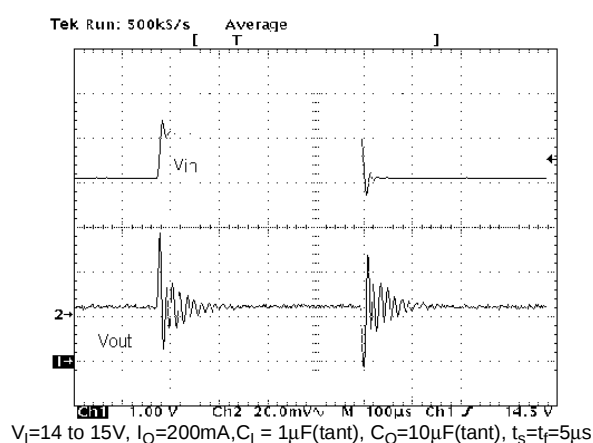
Figure 27: Line Transient
