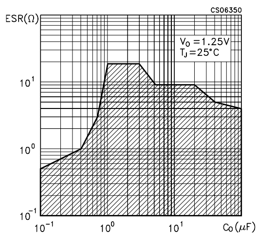
Figure 24: Stability
