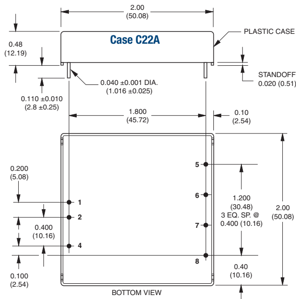
Model BWR-5/3-3.3/4.25-D48A-30721
